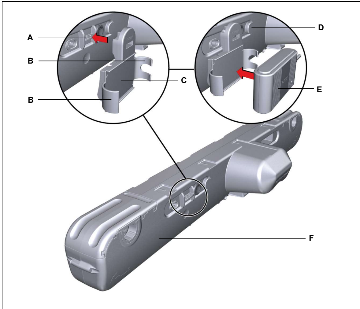
Figure 12 Adapter mount for the RF ECO BT / RF-M-BT
