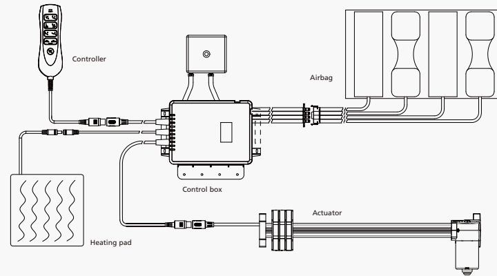
Airbag (FP.17.01) Control Box (CB.16.24) Heating Pad (R5.229.01) Controller (HS.10/HS.16)
